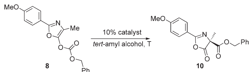
Scheme 4. Enantioselective rearrangement of 8 catalyzed by DMAP derivatives.
