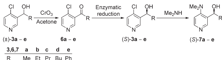
Scheme 3. Preparation of optically active alcohols through a chemical oxidation and enzymatic reduction sequence.
