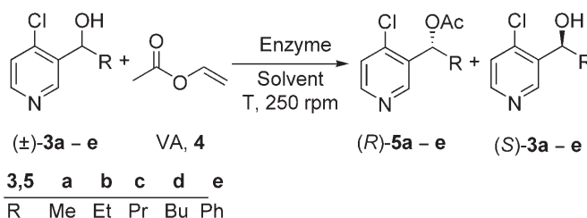
Scheme 2. Kinetic resolution of (±)- 3a–e by lipase-catalyzed transesterification.
